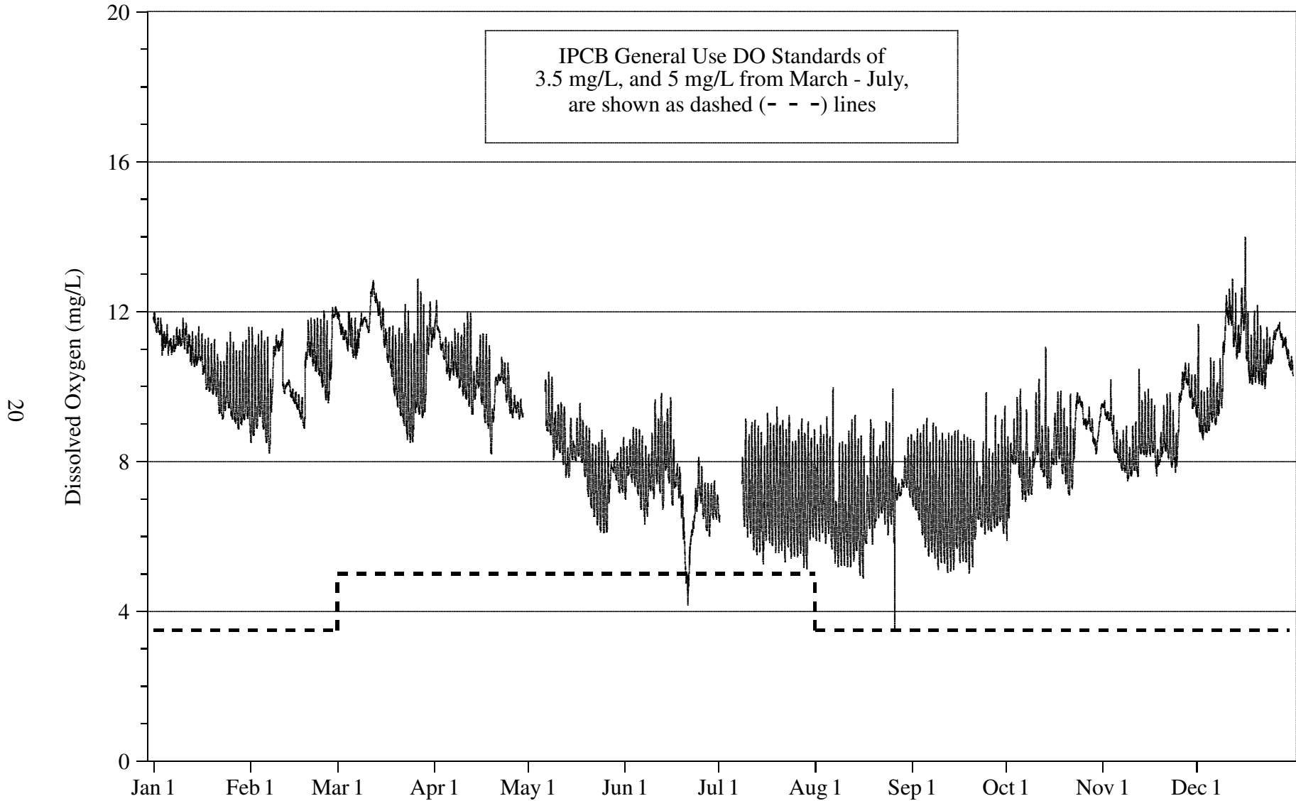
FIGURE 8: DISSOLVED OXYGEN CONCENTRATION MEASURED HOURLY AT JFK BOULEVARD ON SALT CREEK FROM JANUARY 1, 2009, THROUGH DECEMBER 31, 2009
