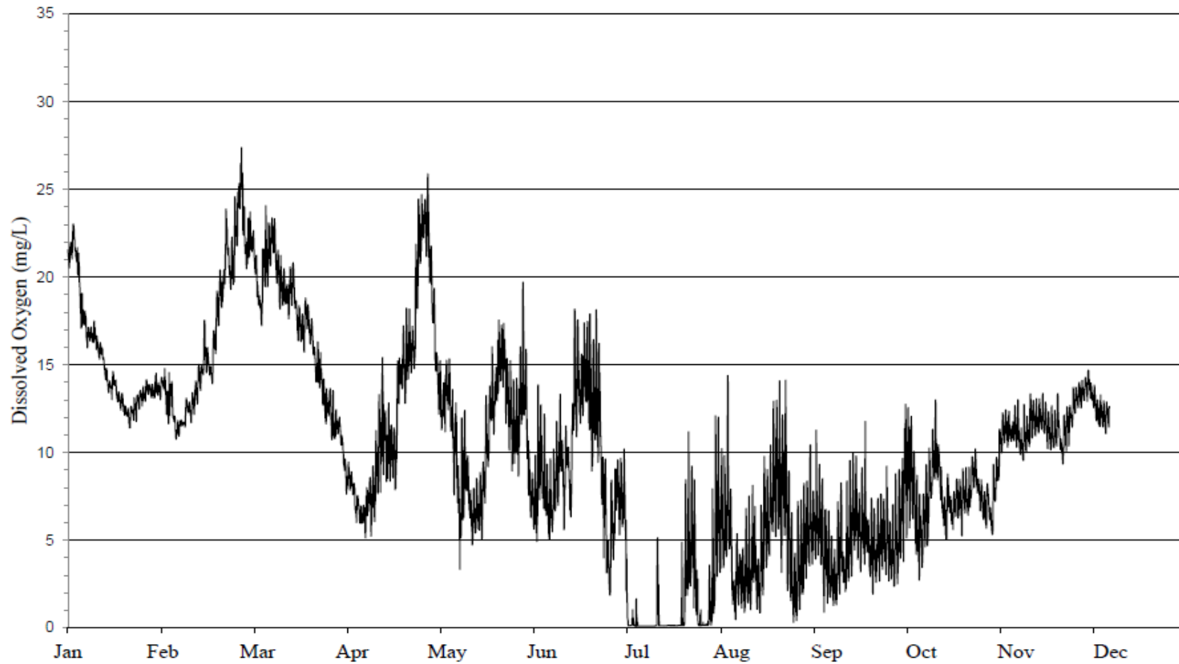
FIGURE 8: DISSOLVED OXYGEN CONCENTRATION MEASURED HOURLY AT 36 TH STREET ON BUBBLY CREEK FROM JANUARY 1, 2023, THROUGH DECEMBER 31, 2023
