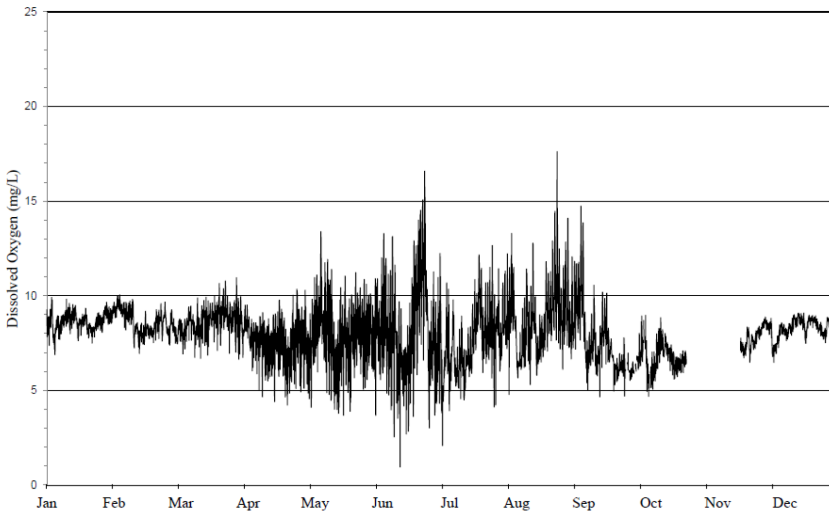
FIGURE 14: DISSOLVED OXYGEN CONCENTRATION MEASURED HOURLY AT HALSTED STREET ON THE LITTLE CALUMET RIVER FROM JANUARY 1, 2023, THROUGH DECEMBER 31, 2023
