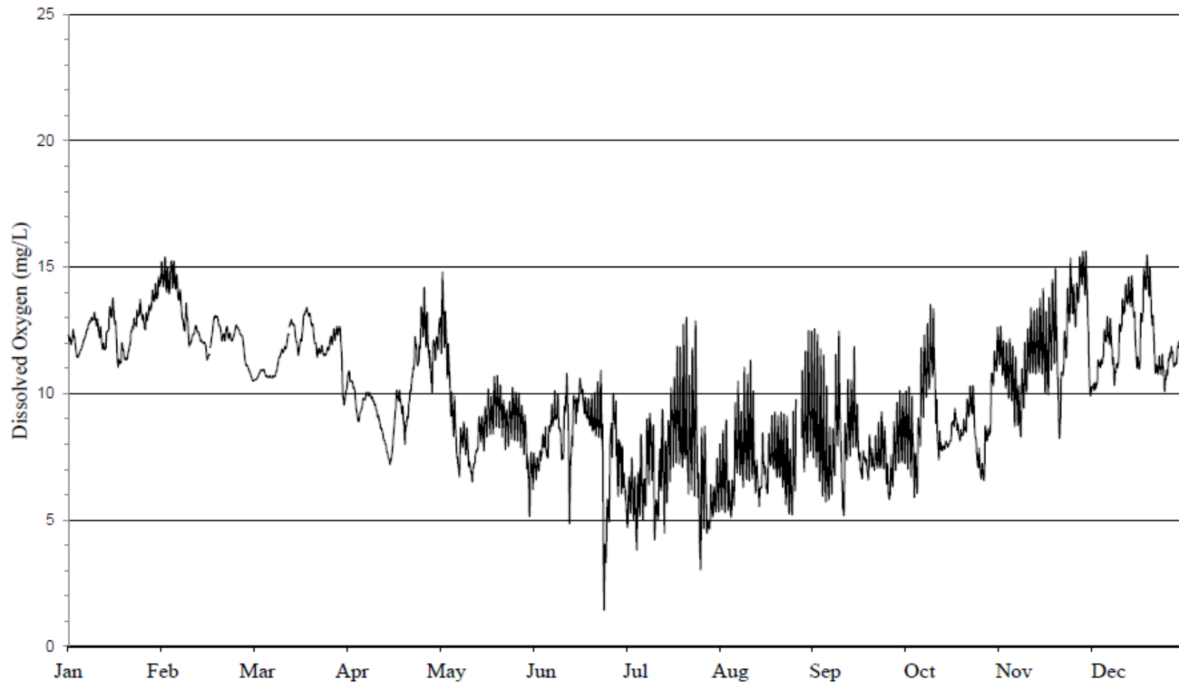
FIGURE 18: DISSOLVED OXYGEN CONCENTRATION MEASURED HOURLY AT DEVON AVENUE ON THE DES PLAINES RIVER FROM JANUARY 1, 2023, THROUGH DECEMBER 31, 2023
