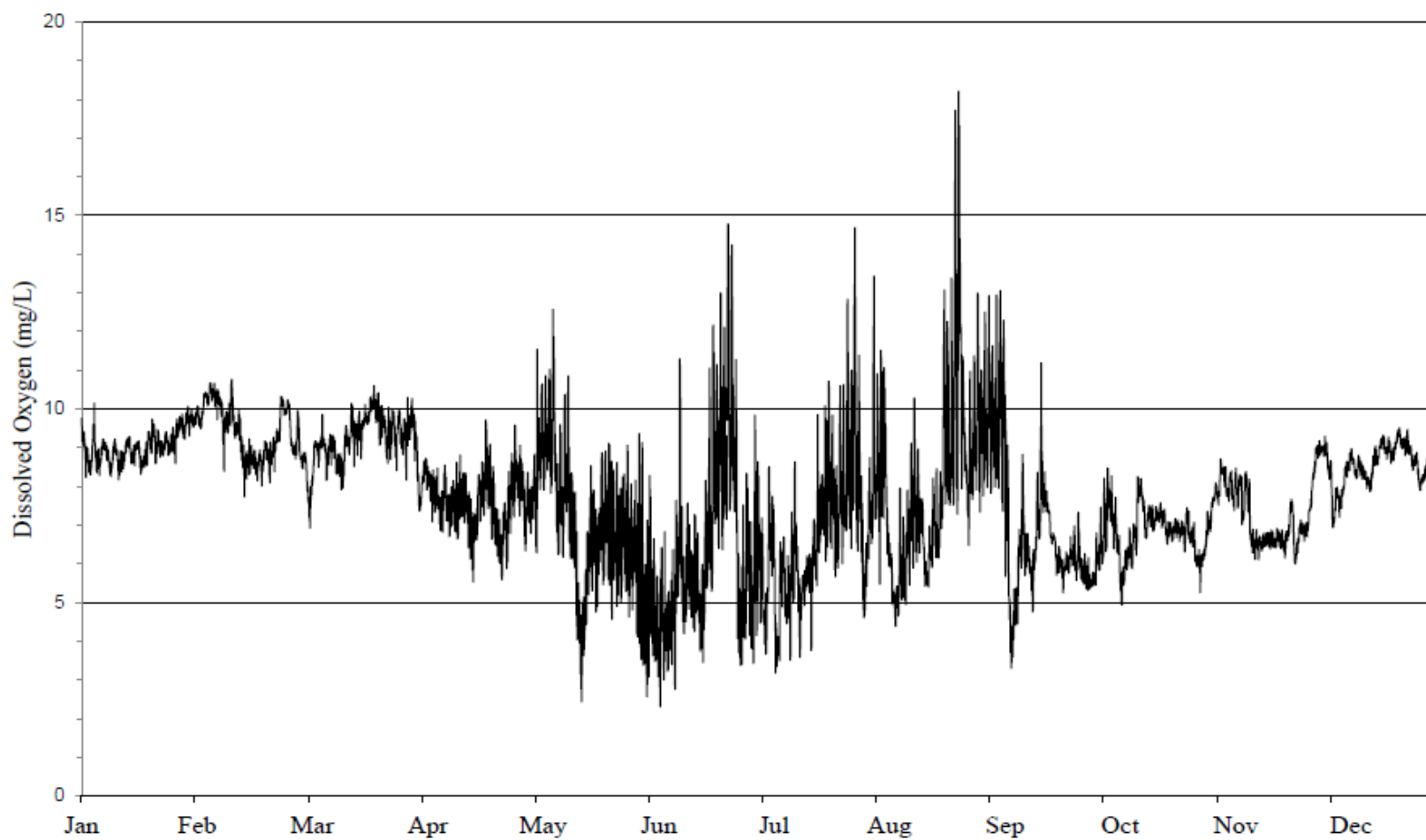
FIGURE 16: DISSOLVED OXYGEN CONCENTRATION MEASURED HOURLY AT CICERO AVENUE ON THE CALUMET- SAG CHANNEL FROM JANUARY 1, 2023, THROUGH DECEMBER 31, 2023
