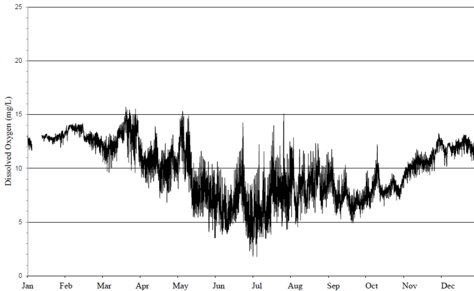
FIGURE 13: DISSOLVED OXYGEN CONCENTRATION MEASURED HOURLY AT THE CHICAGO AND WESTERN INDIANA RAILROAD ON THE LITTLE CALUMET RIVER FROM JANUARY 1, 2023, THROUGH DECEMBER 31, 2023
