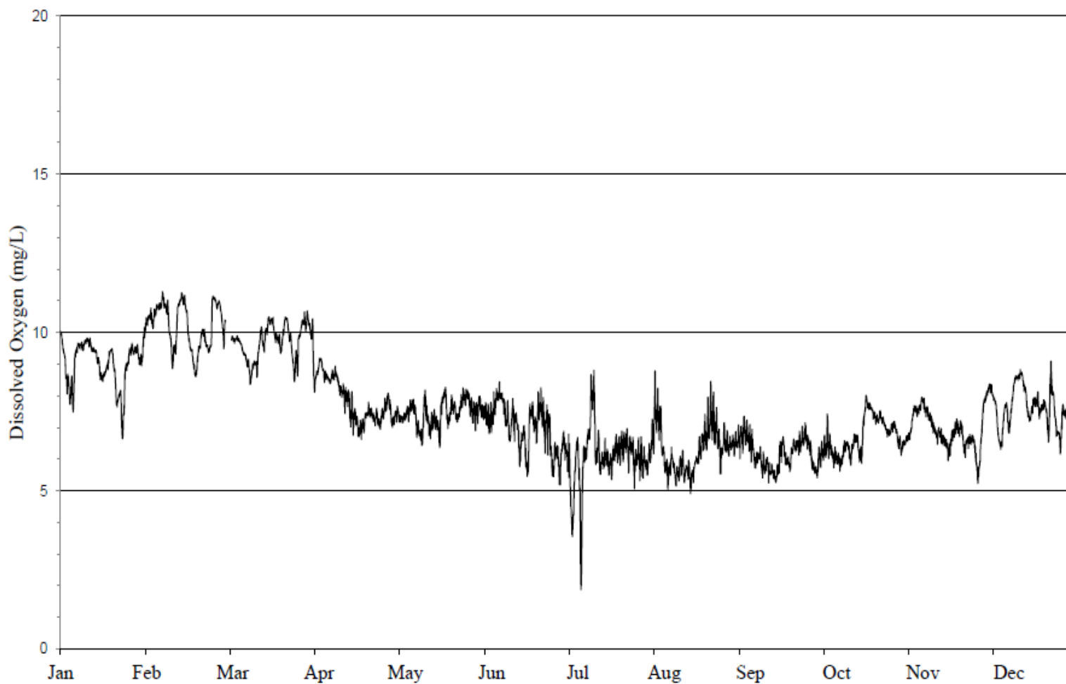
FIGURE 7: DISSOLVED OXYGEN CONCENTRATION MEASURED HOURLY AT LOOMIS STREET ON THE SOUTH BRANCH OF THE CHICAGO RIVER FROM JANUARY 1, 2023, THROUGH DECEMBER 31, 2023
