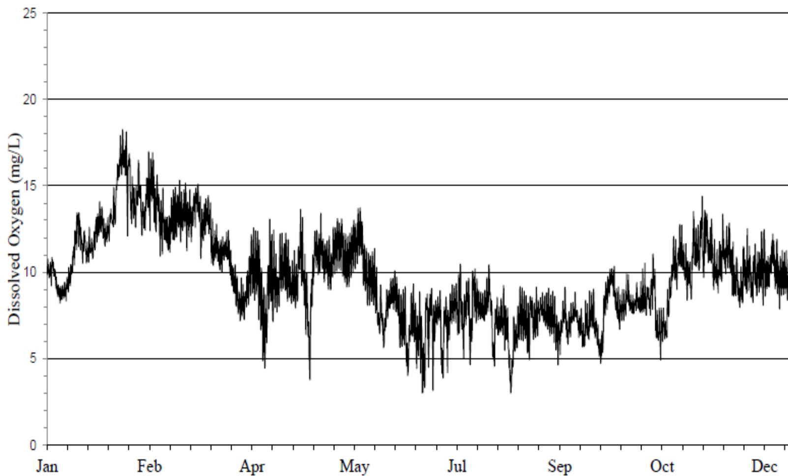
FIGURE 2: DISSOLVED OXYGEN CONCENTRATION MEASURED HOURLY AT CHURCH STREET ON THE NORTH SHORE CHANNEL FROM JANUARY 1, 2023, THROUGH DECEMBER 31, 2023
