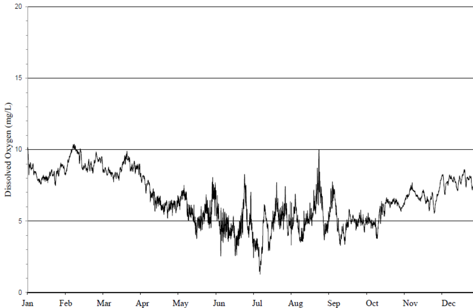
FIGURE 12: DISSOLVED OXYGEN CONCENTRATION MEASURED HOURLY AT LOCKPORT POWERHOUSE ON THE CHICAGO SANITARY AND SHIP CANAL FROM JANUARY 1, 2023, THROUGH DECEMBER 31, 2023
