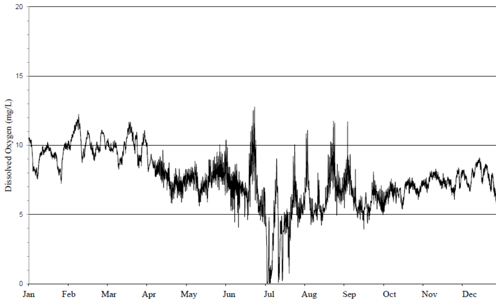
FIGURE 10: DISSOLVED OXYGEN CONCENTRATION MEASURED HOURLY AT CICERO AVENUE ON THE CHICAGO SANITARY AND SHIP CANAL FROM JANUARY 1, 2023, THROUGH DECEMBER 31, 2023
