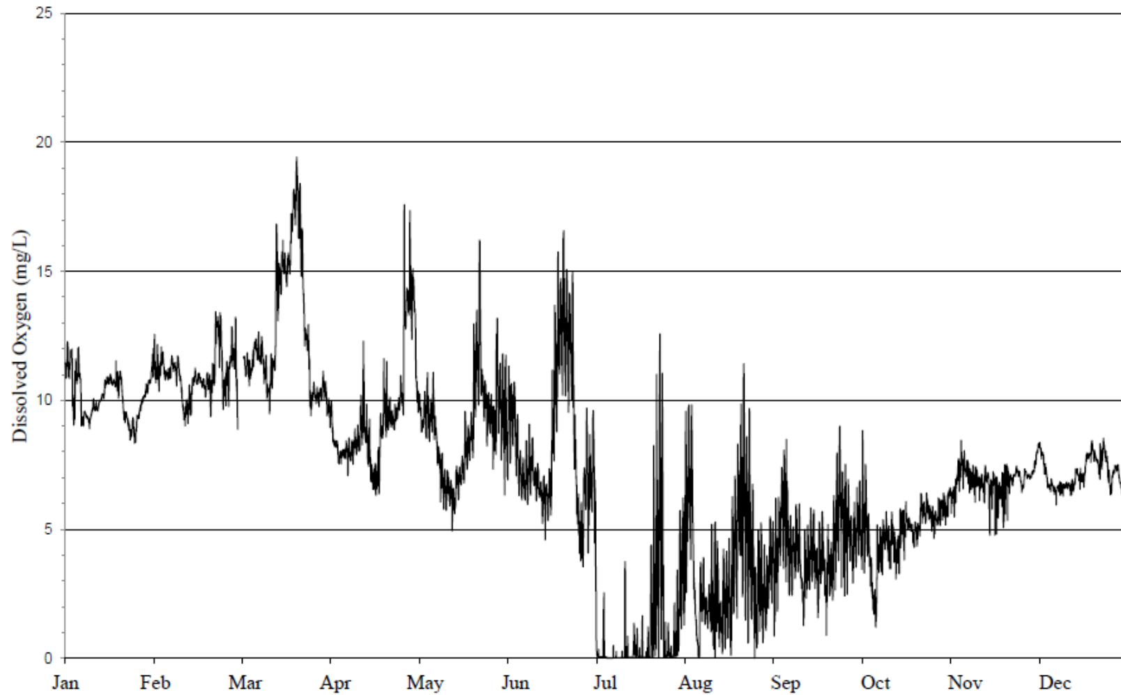
FIGURE 9: DISSOLVED OXYGEN CONCENTRATION MEASURED HOURLY AT INTERSTATE HIGHWAY 55 ON BUBBLY CREEK FROM JANUARY 1, 2023, THROUGH DECEMBER 31, 2023
