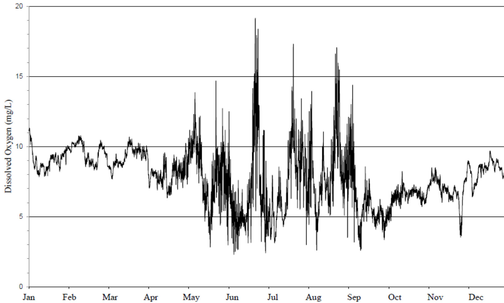
FIGURE 17: DISSOLVED OXYGEN CONCENTRATION MEASURED HOURLY AT ROUTE 83 ON THE CALUMET-SAG CHANNEL FROM JANUARY 1, 2023, THROUGH DECEMBER 31, 2023
