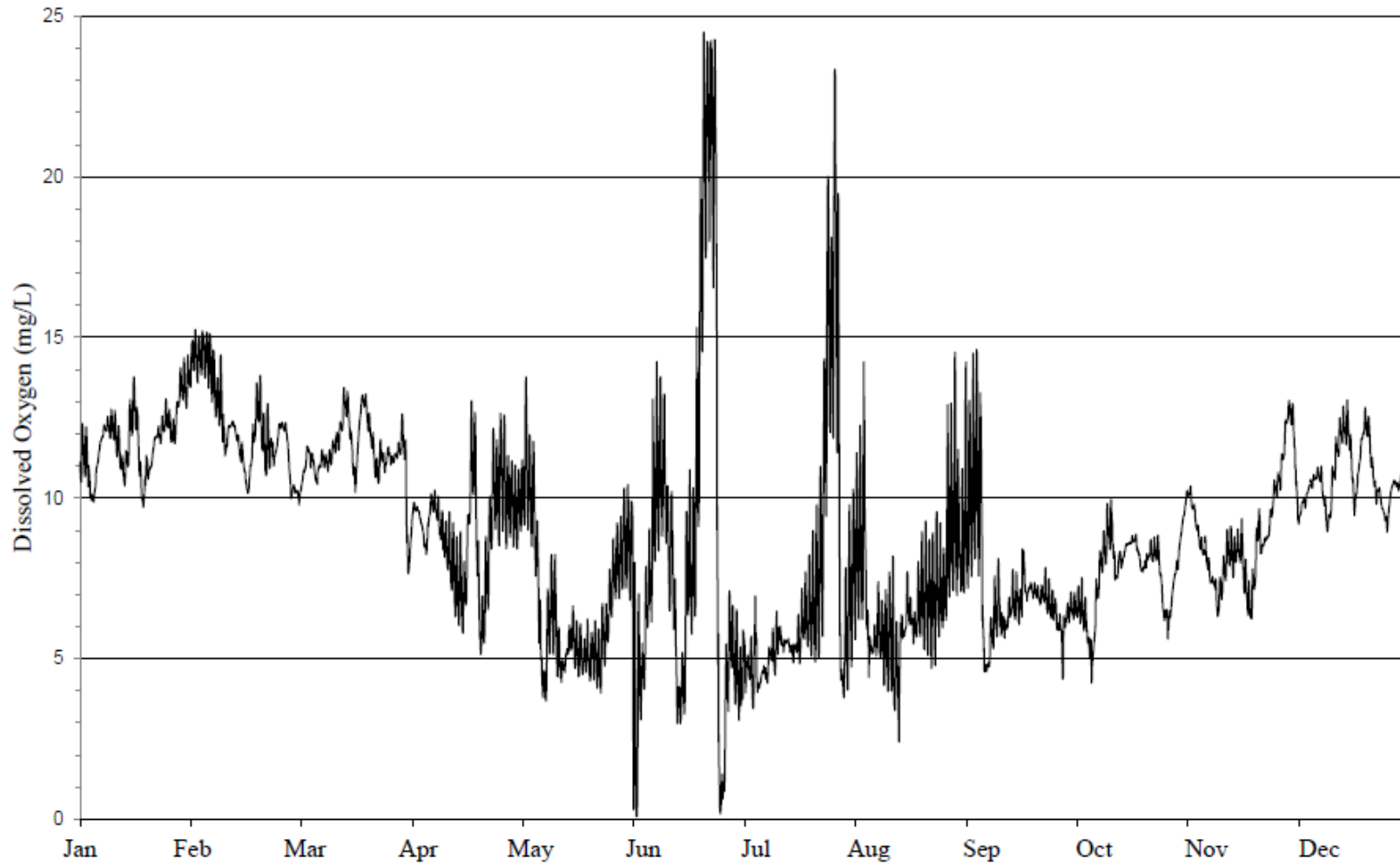
FIGURE 15: DISSOLVED OXYGEN CONCENTRATION MEASURED HOURLY AT ASHLAND AVENUE ON THE LITTLE CALUMET RIVER FROM JANUARY 1, 2023, THROUGH DECEMBER 31, 2023
