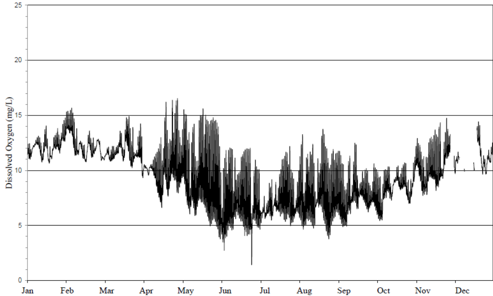
FIGURE 21: DISSOLVED OXYGEN CONCENTRATION MEASURED HOURLY AT WOLF ROAD ON SALT CREEK FROM JANUARY 1, 2023, THROUGH DECEMBER 31, 2023
