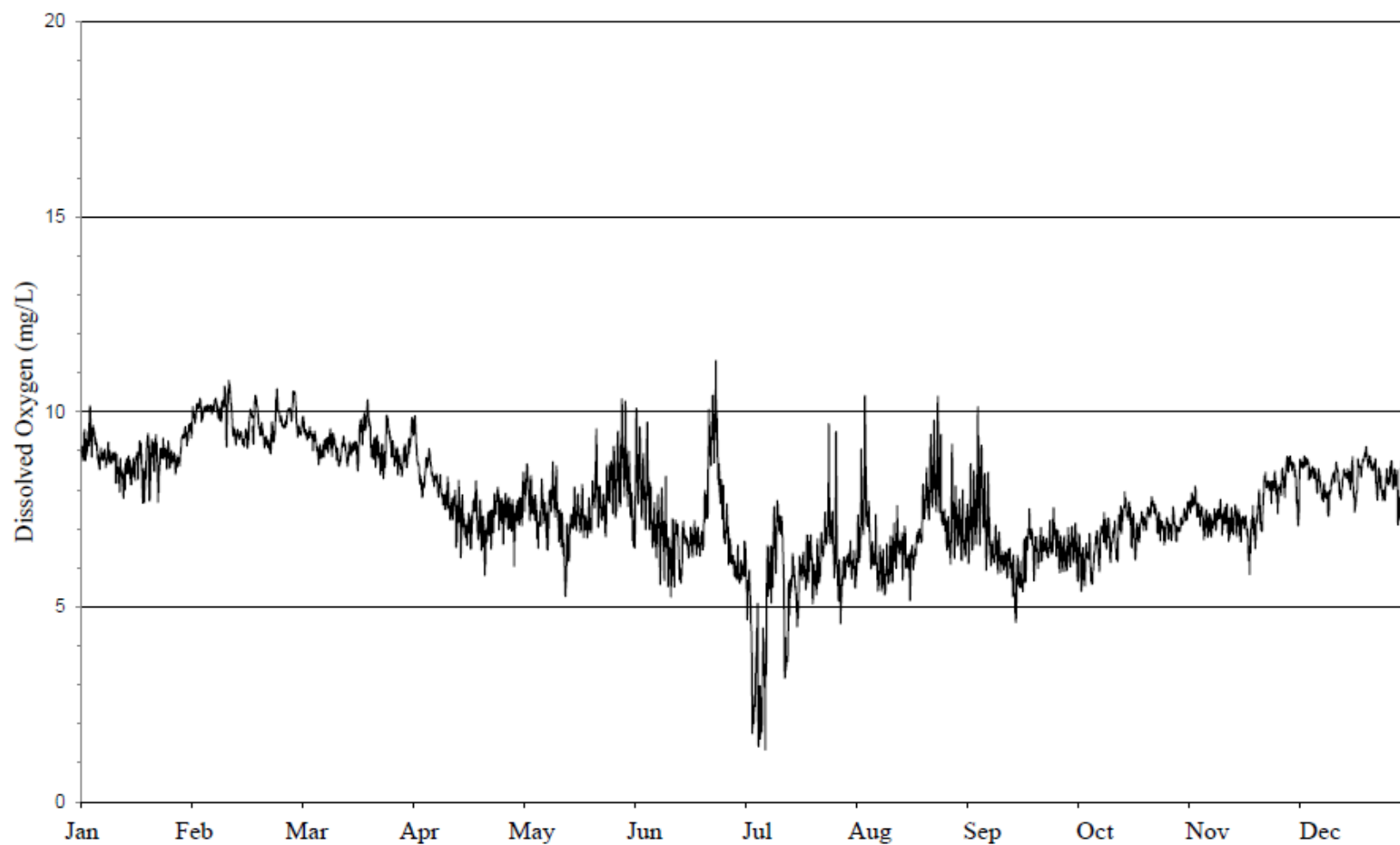
FIGURE 11: DISSOLVED OXYGEN CONCENTRATION MEASURED HOURLY AT THE BALTIMORE & OHIO RAILROAD ON THE SANITARY AND SHIP CANAL FROM JANUARY 1, 2023, THROUGH DECEMBER 31, 2023
