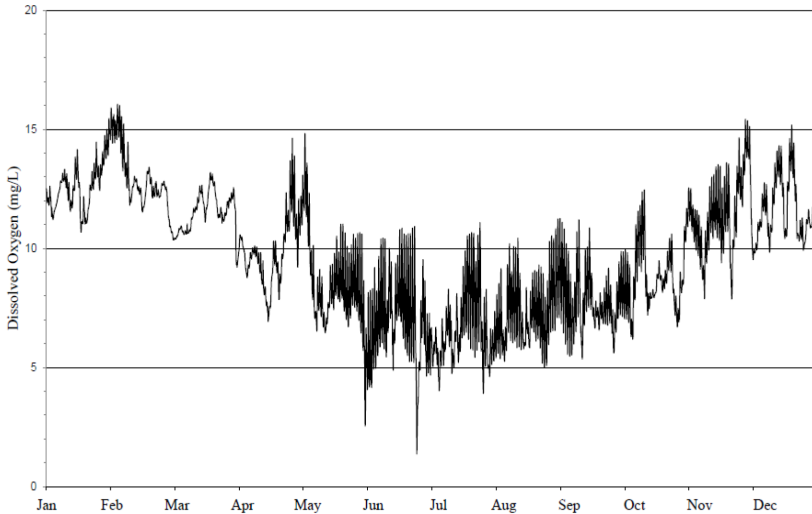
FIGURE 19: DISSOLVED OXYGEN CONCENTRATION MEASURED HOURLY AT IRVING PARK ROAD ON THE DES PLAINES RIVER FROM JANUARY 1, 2023, THROUGH DECEMBER 31, 2023
