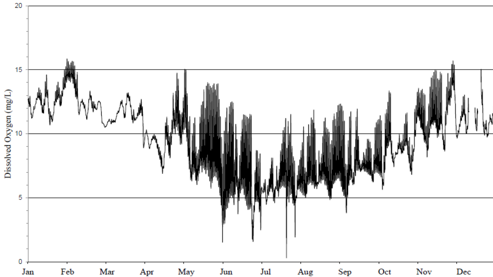
FIGURE 20: DISSOLVED OXYGEN CONCENTRATION MEASURED HOURLY AT OGDEN AVENUE ON THE DES PLAINES RIVER FROM JANUARY 1, 2023, THROUGH DECEMBER 31, 2023
