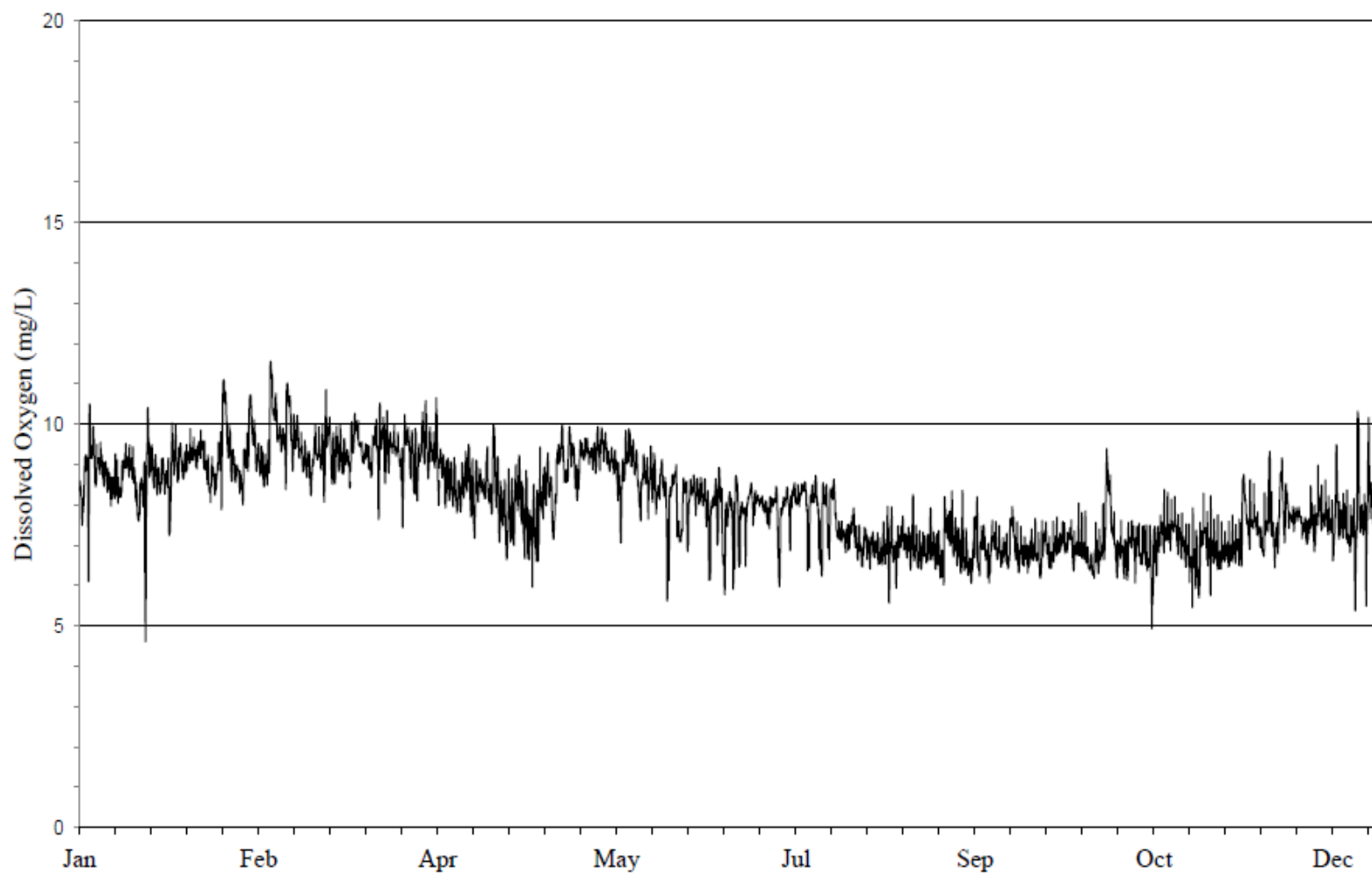
FIGURE 3: DISSOLVED OXYGEN CONCENTRATION MEASURED HOURLY AT FOSTER AVENUE ON THE NORTH SHORE CHANNEL FROM JANUARY 1, 2023, THROUGH DECEMBER 31, 2023
